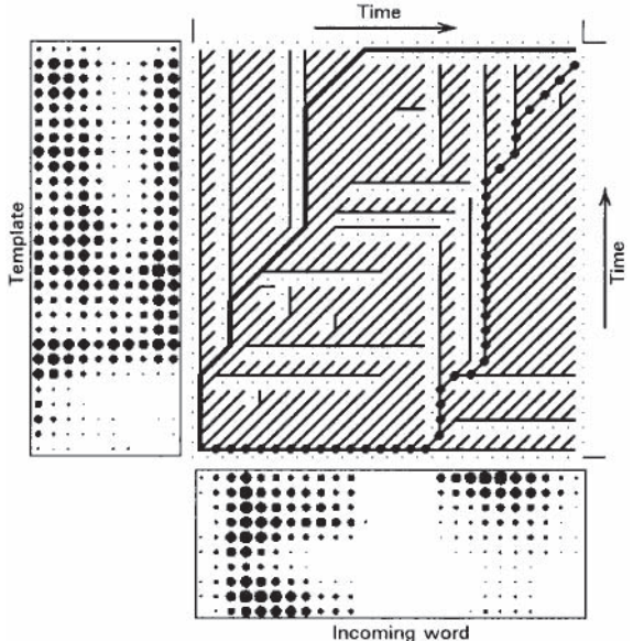
Figure 8.6 The result of trying to align two dissimilar words (“three” and “eight”) within the same DP algorithm as was used for Figure 8.5. The score pruning was removed from this illustration, because any path to the end of the word would then have been seriously sub-optimal. It can be seen that if the last frame had been removed from the template, the path would have been completely different, as marked by blobs.
