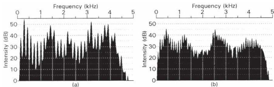
Figure 2.12 Narrow-band spectral cross-sections, taken at the points marked on Figure 2.11.
