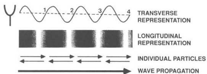
Figure 1: Sinusoidal motion. [From Gelfand (1998), Hearing: An Introduction to Psychological and Physiological Acoustics , Third Edition, New York: Marcel Dekker, Figure 1.5, p. 15, with permission.]
