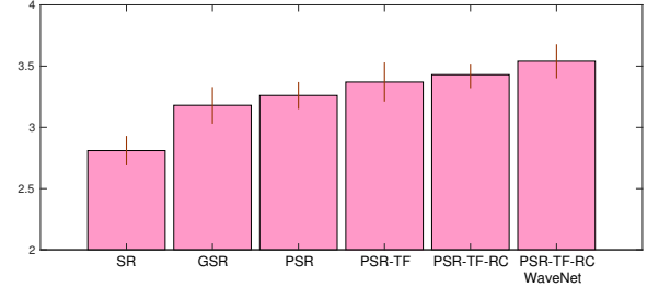
Fig. 10: A comparison of MOS for joint spectrum and prosody conversion over the sparse representation schemes discussed in this paper, that include SR [11], PSR [15], GSR, PSR-TF, PSR-TF-RC and PSR-TF-RC with adapted WaveNet vocoder (PSR-TF-RC-WaveNet).
