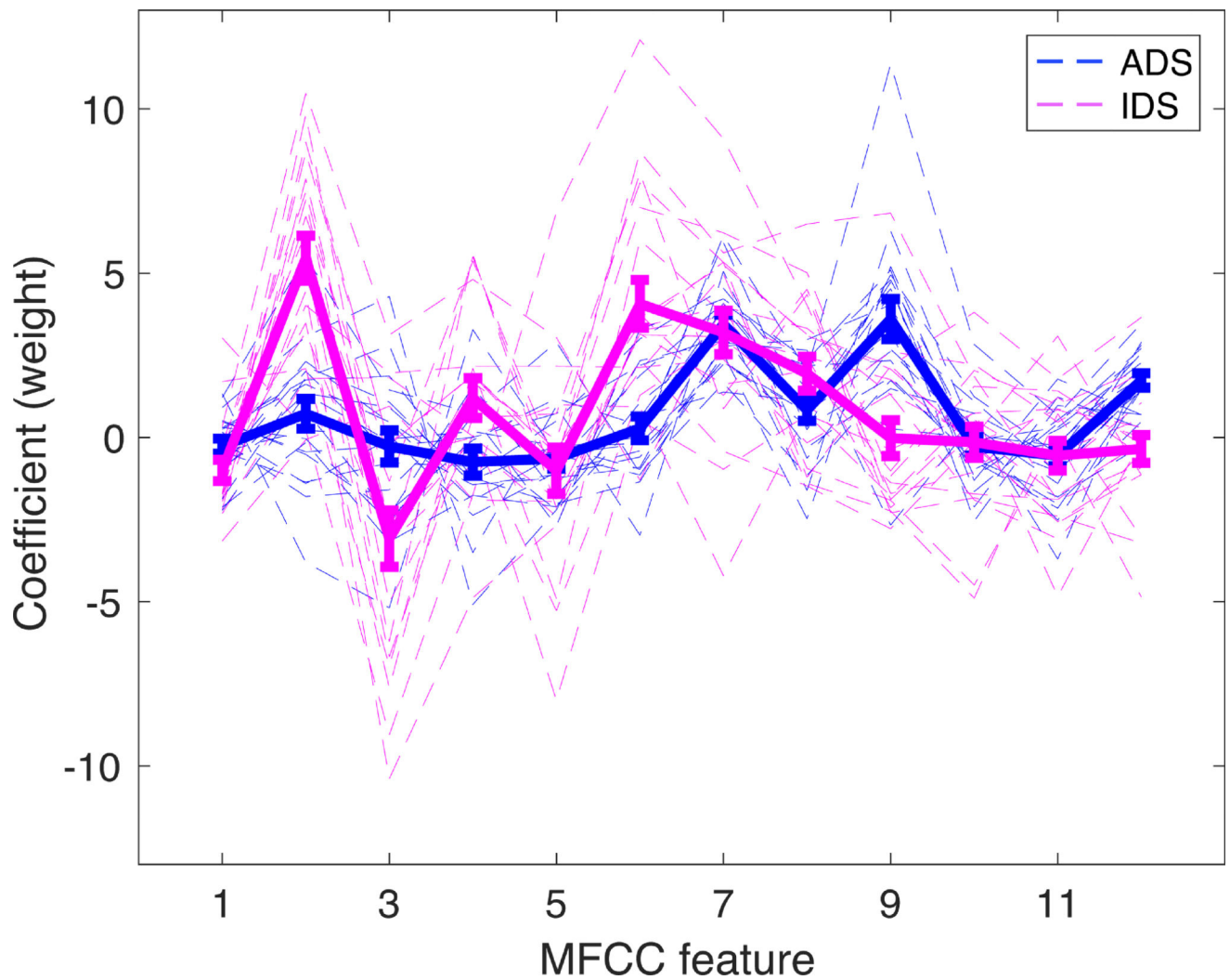
Figure 1. MFCC feature vectors from all utterances for one representative participant Each vector (dashed lines) represents the time-averaged set of Mel-frequency cepstral coefficients for a single utterance of either adult-directed speech (ADS, shown in blue) or infant-directed speech (IDS, shown in pink). Each bold line represents the average MFCC vector across all 20 utterances for a given condition. Error bars on the averaged vectors represent \pm SEM across 20 utterances. Figure S1 depicts average MFCC vectors for each of the 12 English-speaking participants; the vectors displayed in Figure 1 come from s12.
