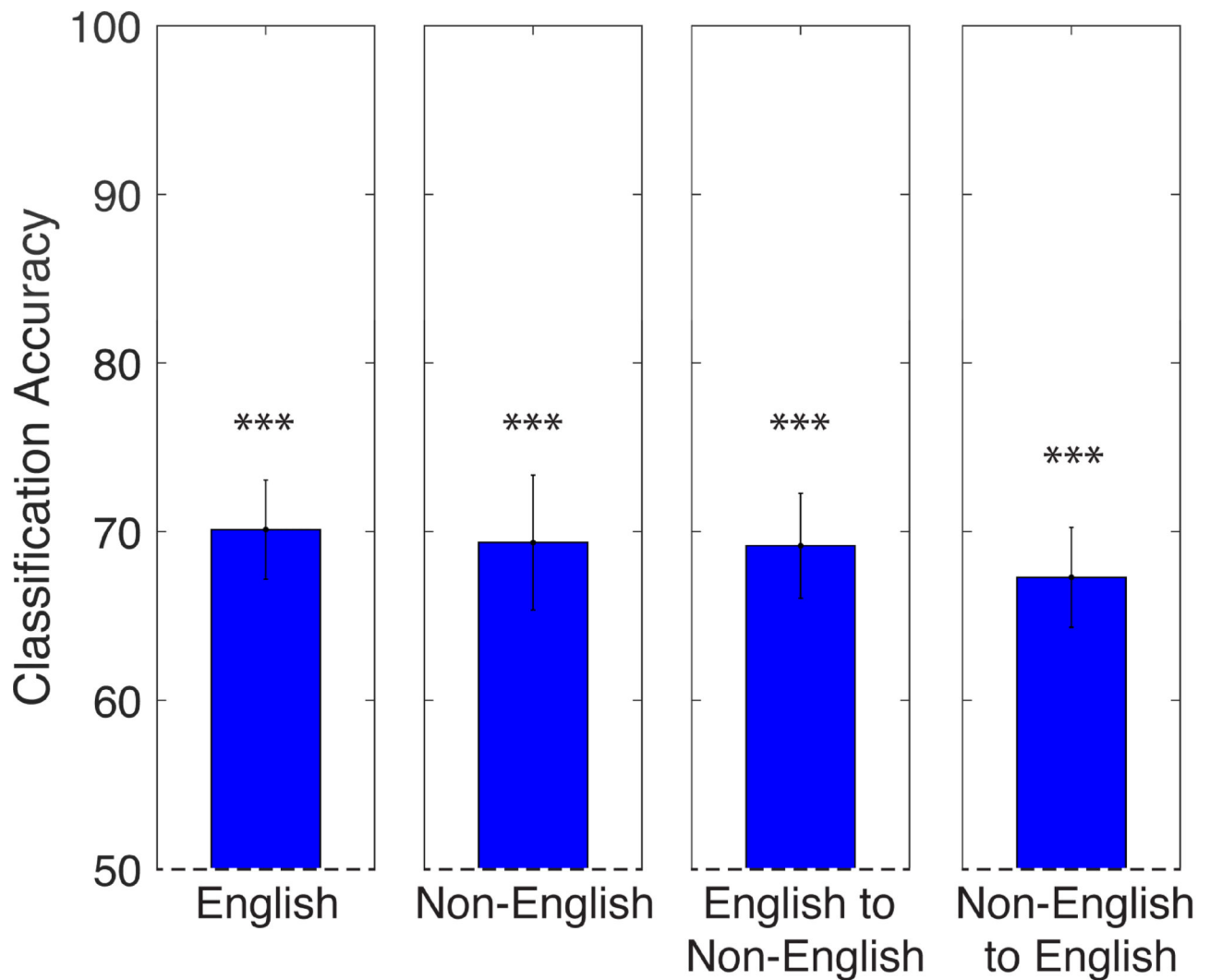
Figure 2. Accuracy rates for classifying mothers' IDS vs. ADS using MFCC vectors
