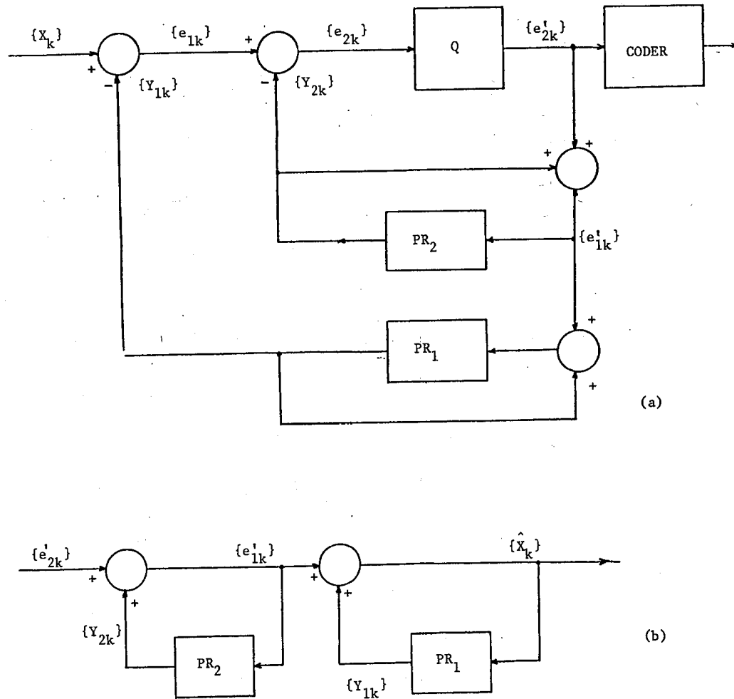
FIGURE 5.7 - A DPCM Codec using Two Separate Predictors.
