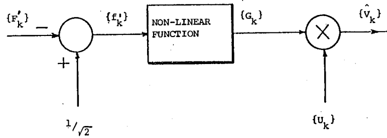
FIGURE 6.14 - The Inverse Non-Linear Element.
