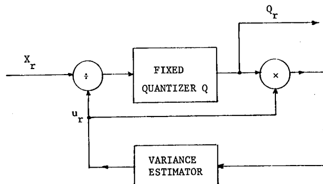
FIGURE 6.5 - The Variance Estimating Adaptive Quantizer.
