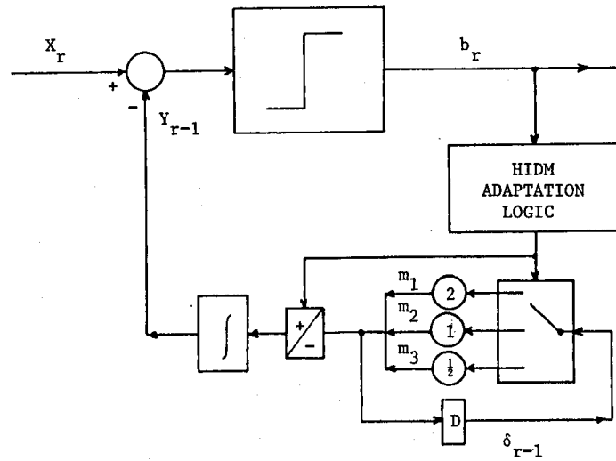
FIGURE 2.13 - The High Information Delta Modulator.
