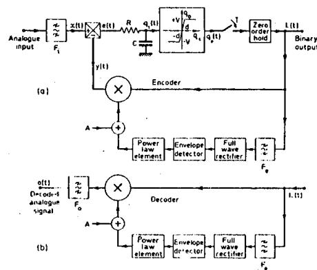
FIGURE 2.19 - The Syllabically Companded DSM (after (2))
