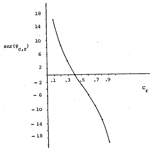
FIGURE 6.15 - \text{snr}(\psi_{c,r}) as a function of C_r .
