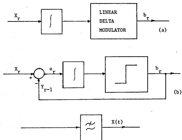
FIGURE 2.12 - (a) The Delta Sigma Modulator (DSM)
