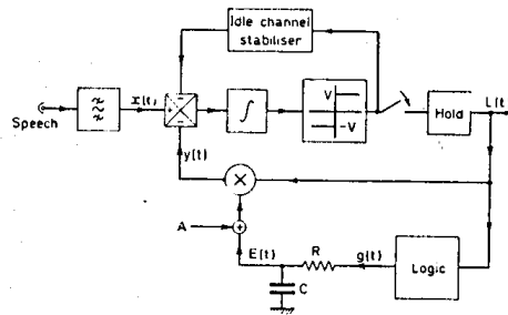
FIGURE 2.18 - The SCALE Encoder (after (2))
