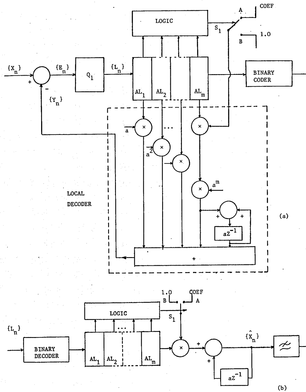
FIGURE 4.13 - The Scheme 2 Delayed DPCM system.
