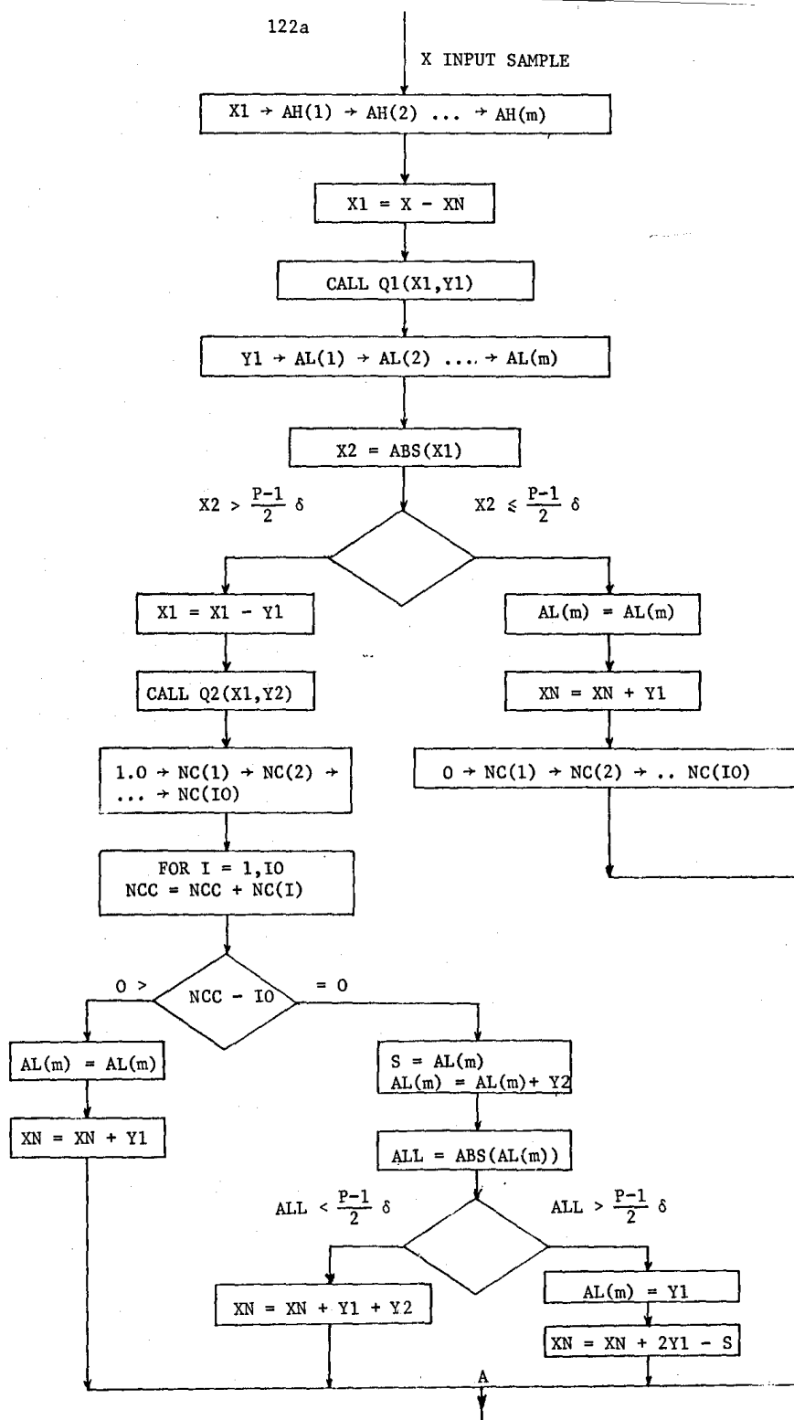
FIGURE 4.8 - Part of Scheme 1 Simulation Procedure.
