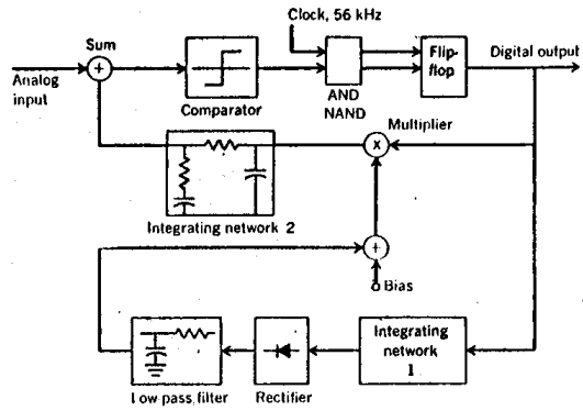
FIGURE 2.16 - Tomozawa's and Kaneko's ADM. (after (108))
