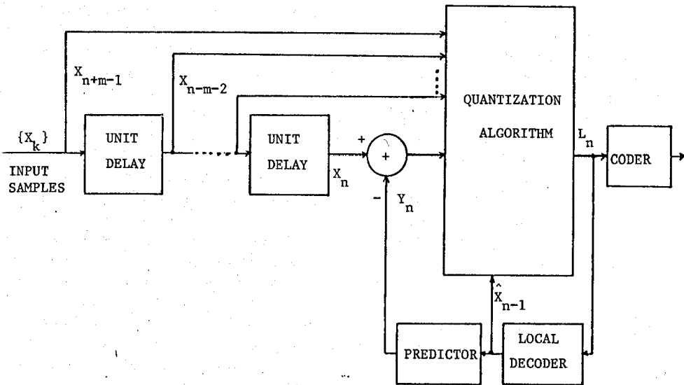
FIGURE 4.1 - Delayed Differential Encoder.
