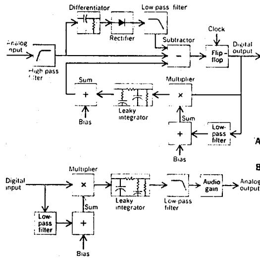
FIGURE 2.15 - The Continuous Delta Modulator (after (108))
