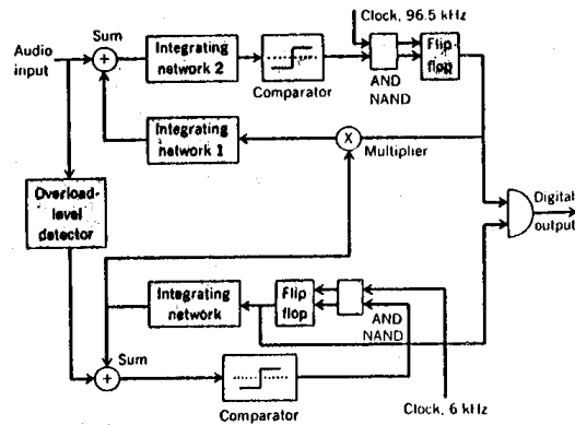
FIGURE 2.17 - Brolin's and Brown's ADM. (after (108))
