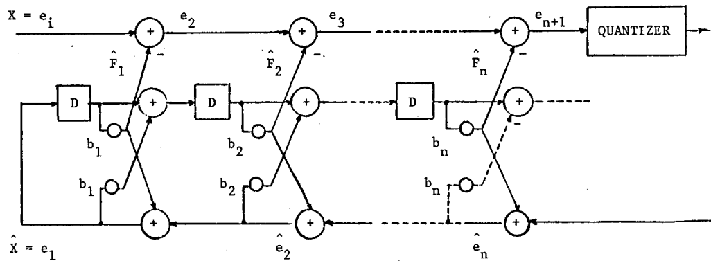
FIGURE 5.3 - A Differential Encoder using the Lattice Predictor.
