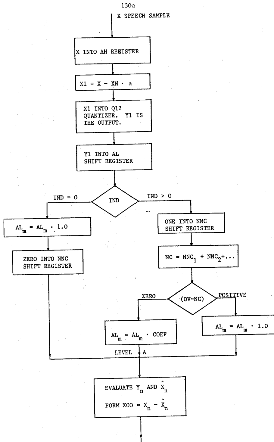
FIGURE 4.14 - Encoding-Decoding Procedure, Scheme 2.
