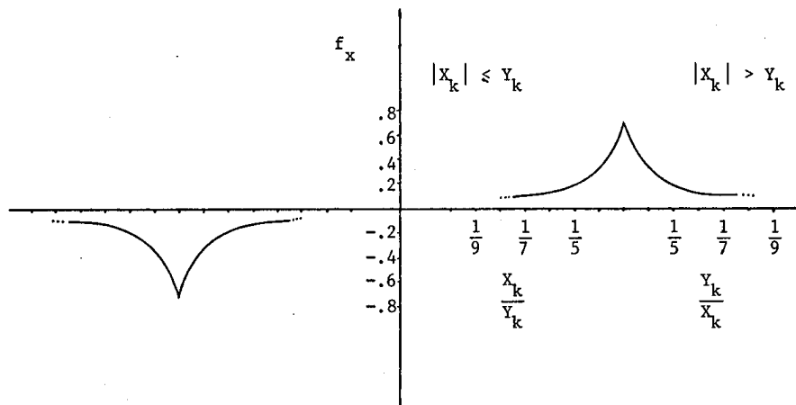
FIGURE 6.8 - The TR Characteristic.
