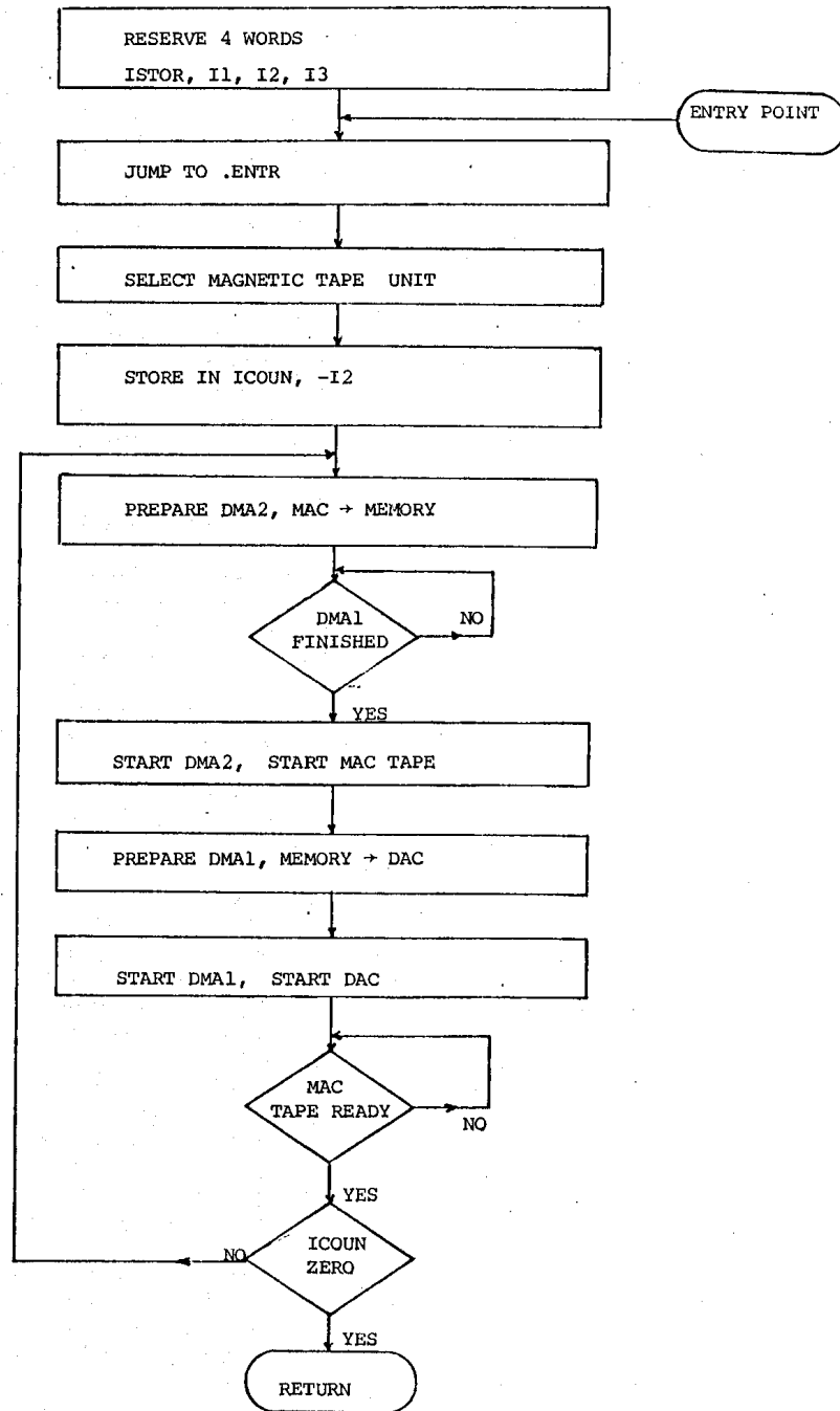
FIGURE 3.14 - Output Operation.
