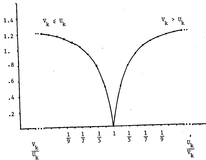
FIGURE 6.13 - Characteristic of the Non-Linear Element.
