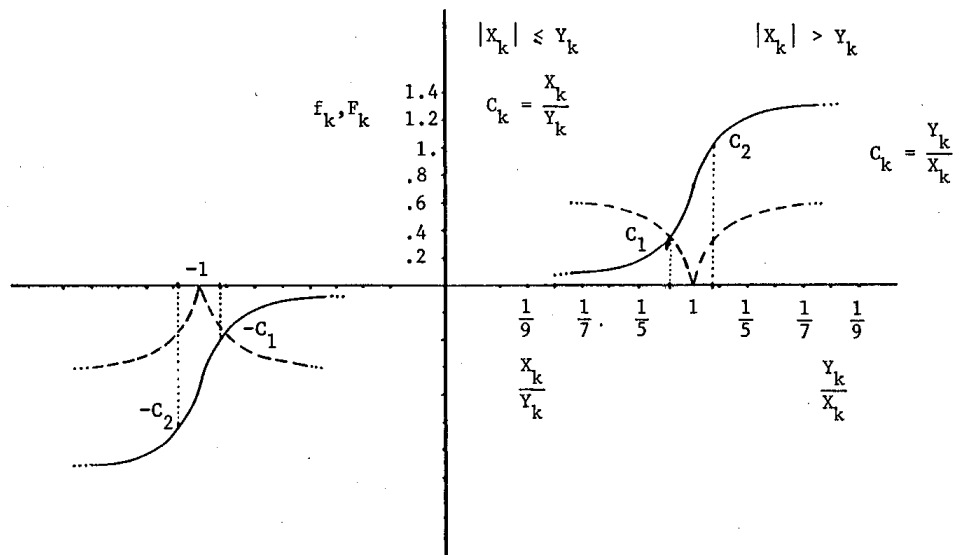
FIGURE 6.9 - The EL and MEL Characteristic.
