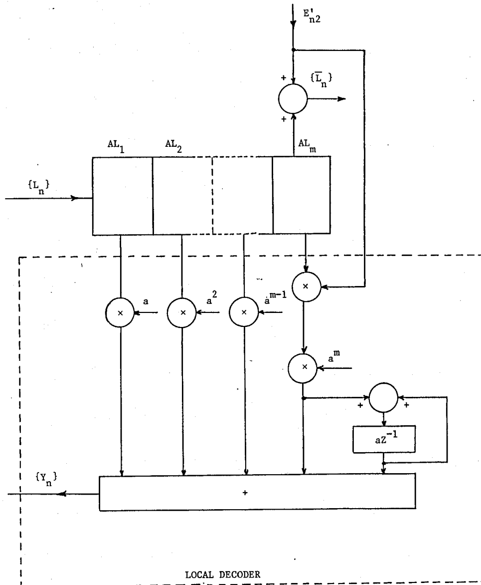
FIGURE 4.5 - The Local Decoder when a < 1 .
