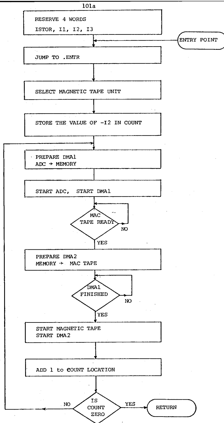
FIGURE 3.13 - Input Operation.
