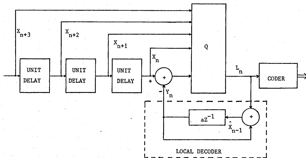
FIGURE 4.2 - Delayed First Order DPCM.
