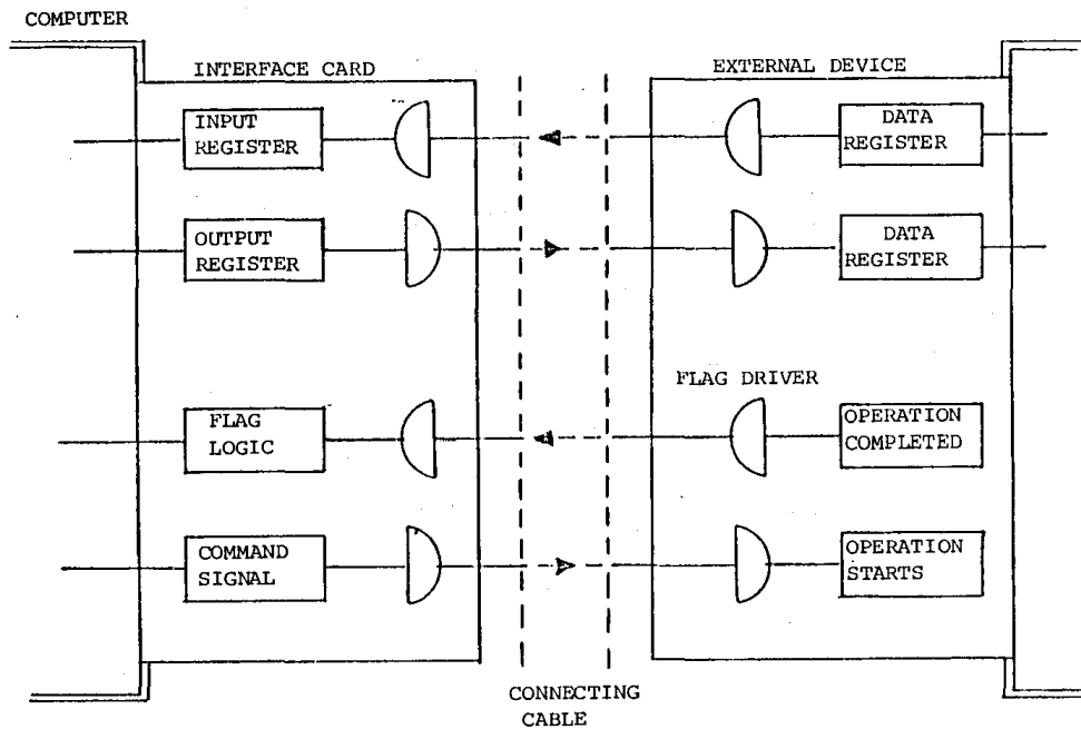
FIGURE 3.2 - Interfacing the Computer with an External Peripheral.
