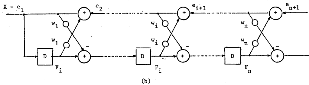
FIGURE 5.2 - (a) The Maximum likelihood Vocoder Filter, (b) Its Inverse Filter.
