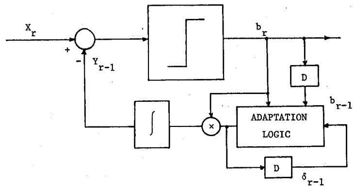
FIGURE 2.14 - Jayant's Adaptive Delta Modulator.
