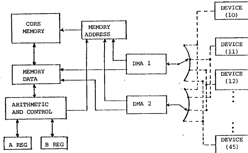
FIGURE 3.1 - Input/Output Data Transfers.
