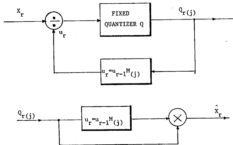
FIGURE 6.2 - Jayant's Adaptive Quantizer.
