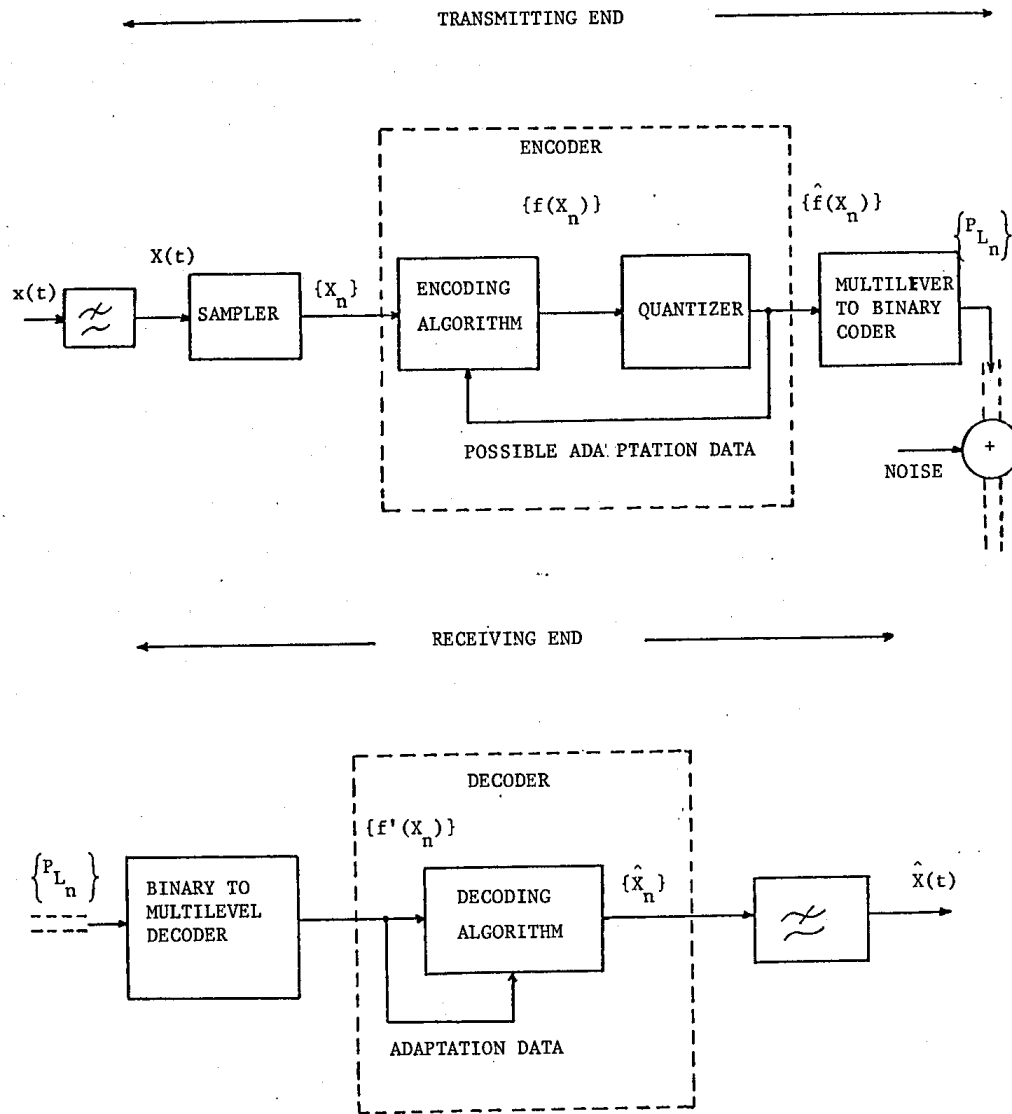
FIGURE 2.7 - Generalized Block Diagram of a Digital Waveform Encoding System.
