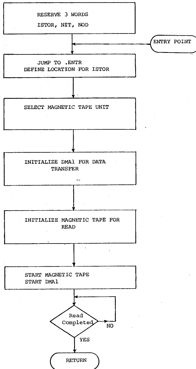
FIGURE 3.10 - Transfer of Data from Magnetic Tape into the Computer.
