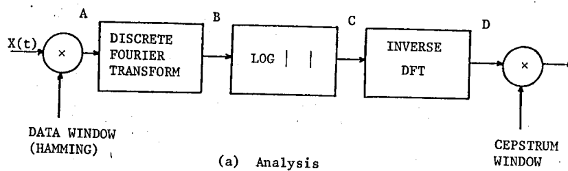
FIGURE 2.3 - A Homomorphic Processing System.
