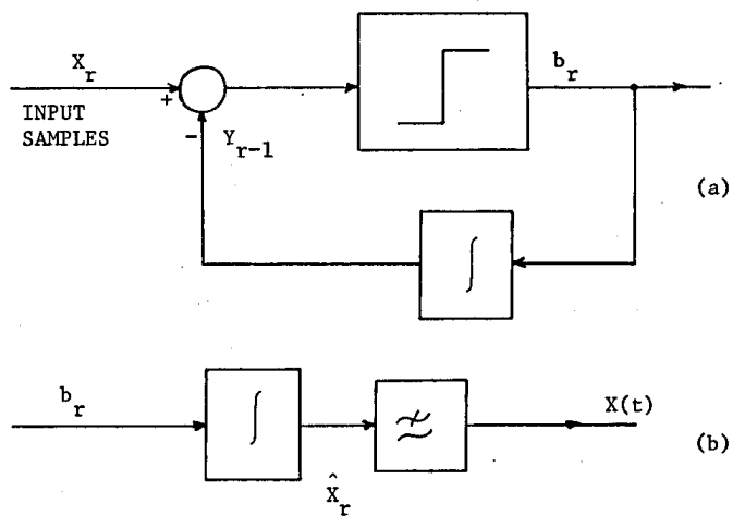
FIGURE 2.11 - The Linear Delta Modulator
