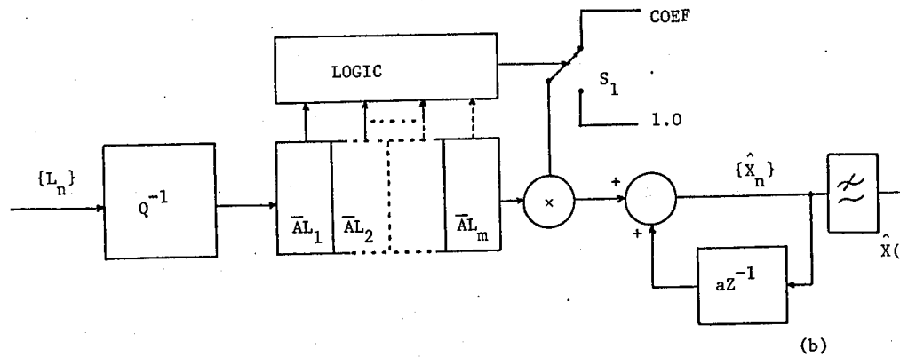
FIGURE 4.17 - Delayed ADPCM, Scheme 2.
