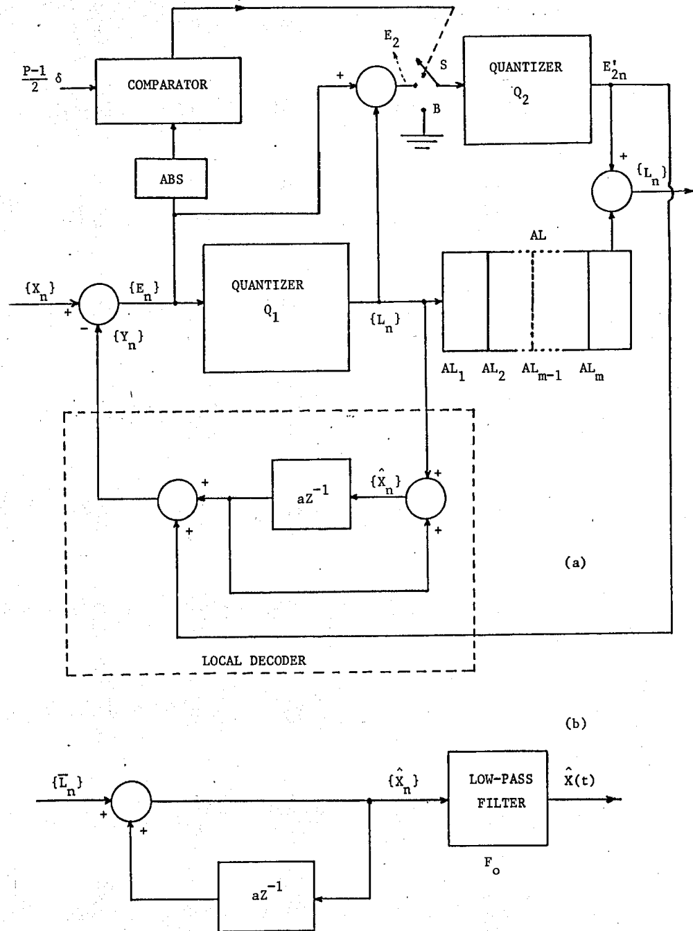
FIGURE 4.4 - Delayed DPCM Codec, Scheme 1.
