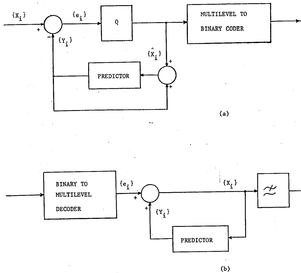
FIGURE 5.1 - The DPCM Codec.
