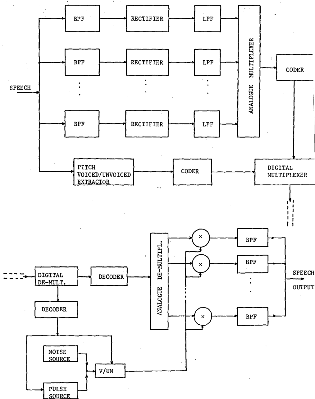
FIGURE 2.2 - A Typical Channel Vocoder.
