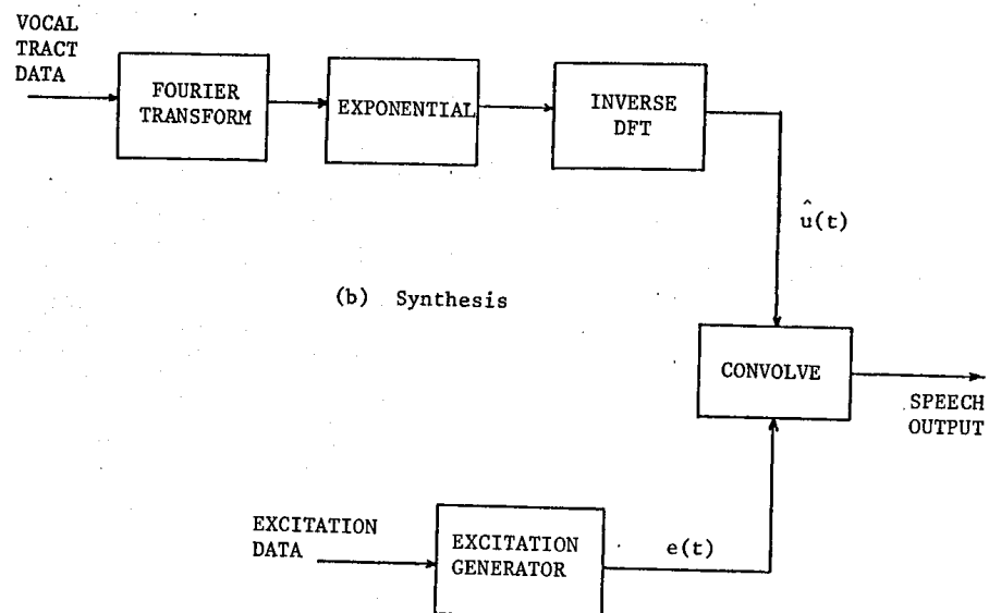
FIGURE 2.4 - The Homomorphic Vocoder.
