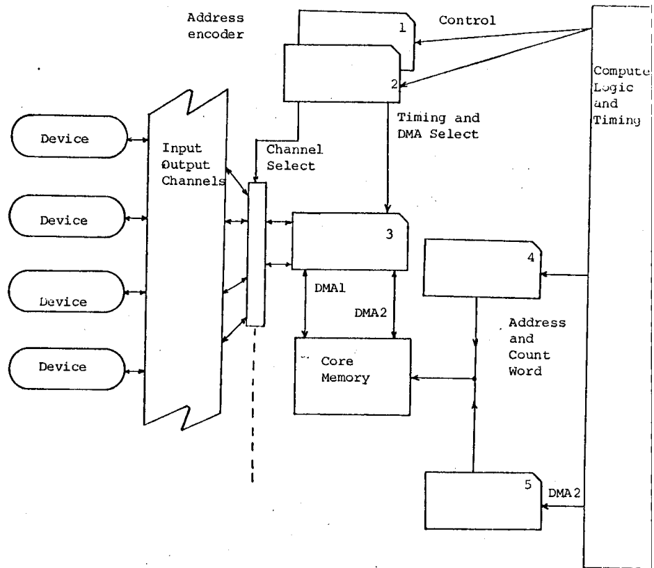
FIGURE 3.9 - DMA Hardware.
