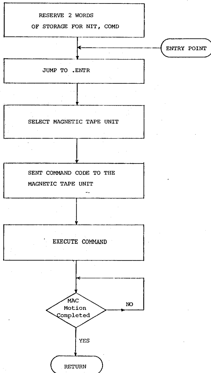
FIGURE 3.12 - The COMMD Subroutine.
