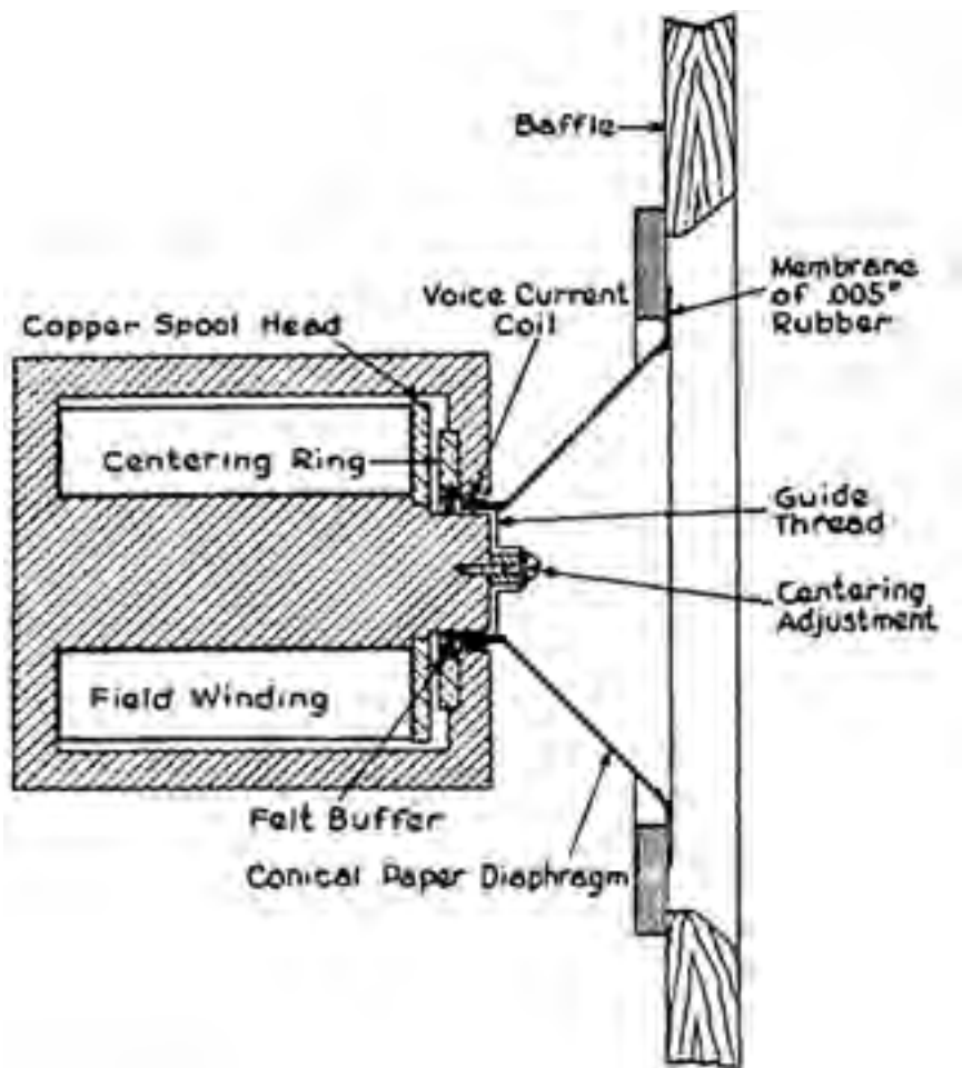
Figure 2.1 A moving coil loudspeaker as developed by Chester W. Rice and Edward W. Kellogg (Rice and Kellogg 1925, 470).
