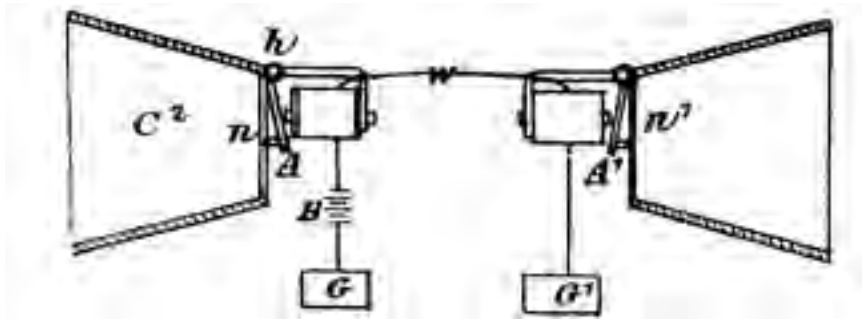
Figure 3.4 Design of two identical devices for transforming sound into electricity that use single metal plates instead of many rods (Bell 1878, 22).
