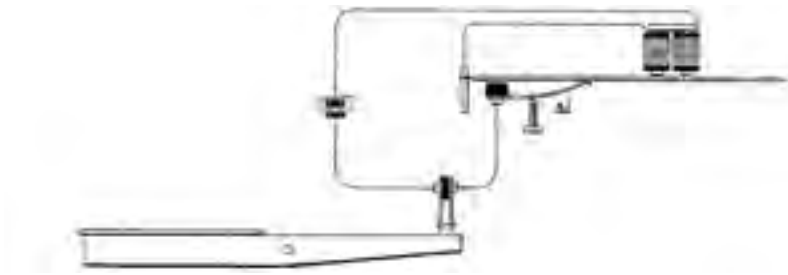
Figure 3.7 The piano string serves as its own current interrupter. When the string vibrates the connection between string and contact-spring M is opened and closed (Dieckmann 1887, 3).
