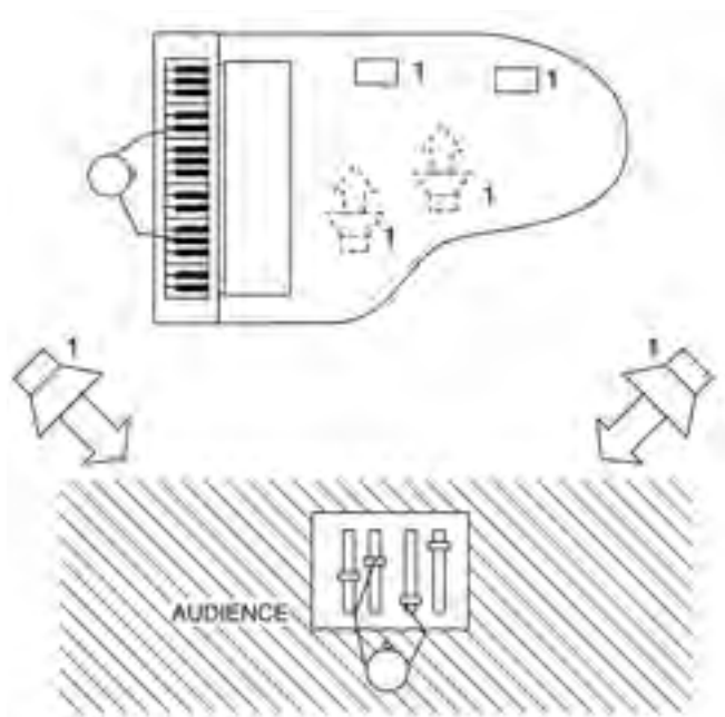
Scheme 4.19 Luigi Nono ..... sofferte onde serene ...: the monophonic tape in this piece can be played through two loudspeakers in the hall as well as through two loudspeakers underneath the grand piano. The person at the mixing desk has to ‘play’ the tape by deciding through which loudspeakers the tape is sounding. Alvis Vidolin added two tactile transducers to have better frequency response for especially the high pitches.
