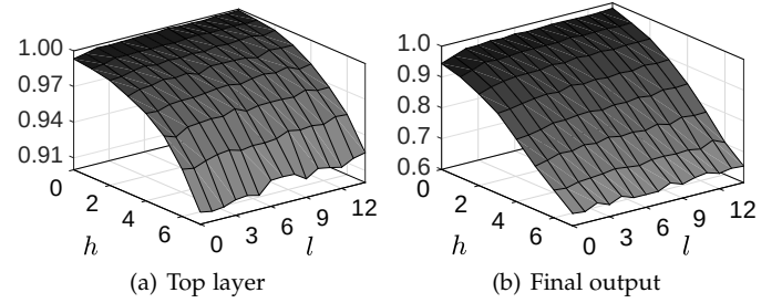
Fig. 8. Reliability of the protected implementation for different number of masked challenge bits h = w(p) and number of repeats l .
