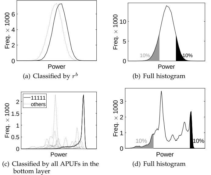
Fig. 4. SCA of the bottom layer of original (1, 5)-IPUF using 100 000 averaged signals, histograms at the point of interest identified in Figure 2(b).
