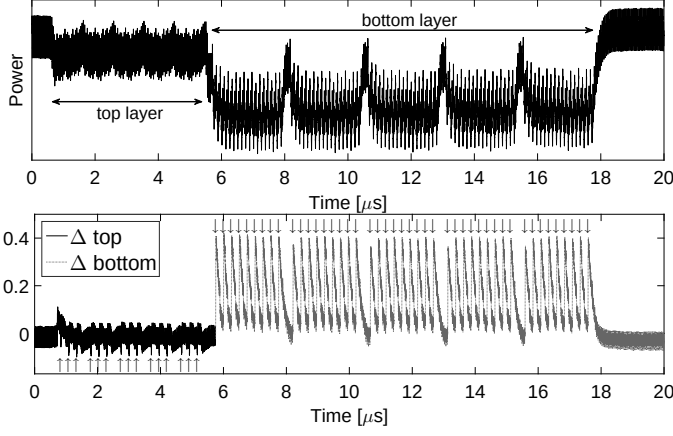
Fig. 9. SCA of our protected (1, 5)-IPUF, 100 000 averaged signals, each of which obtained by repeating 1000 times, (top) an averaged signal, (bottom) difference of means.
