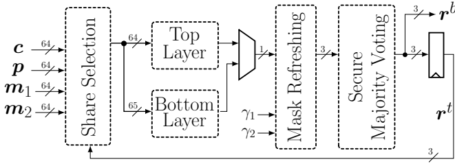
Fig. 7. Application of our construction on Interpose PUF.
