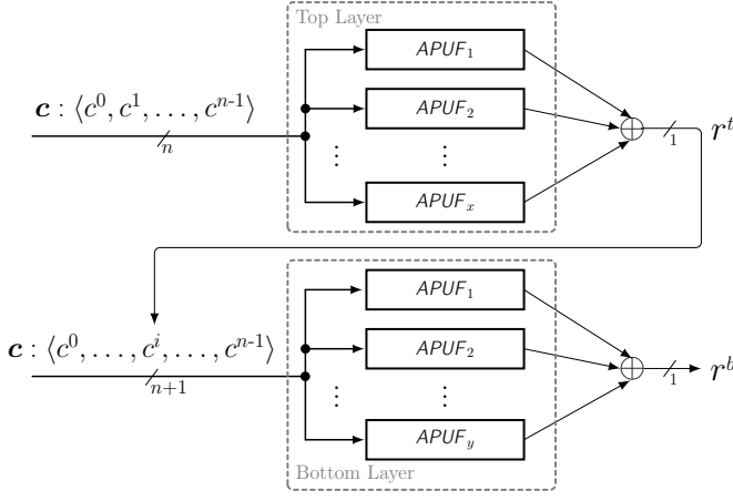
Fig. 1. (x, y) -IPUF.
