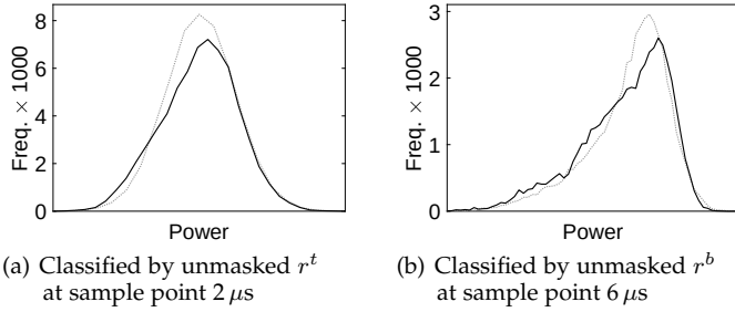
Fig. 10. SCA of our protected (1, 5)-IPUF using 100 000 averaged signals, histograms at an exemplary point of interest identified in Figure 9.
