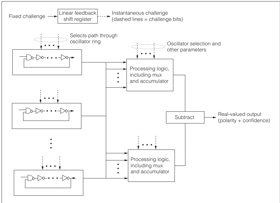
Figure 1. Real-valued physical unclonable function (RV-PUF) using an oscillator and arbiter hybrid approach.
