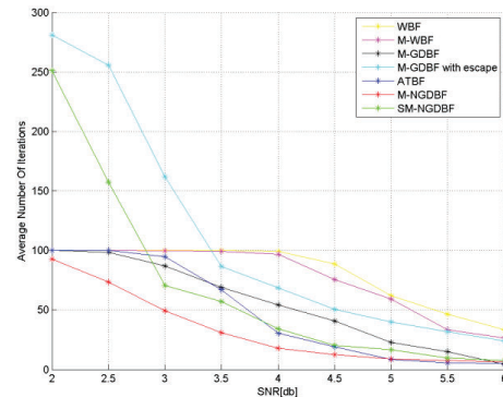
Fig 4. Average number of iterations of bit flipping algorithms: regular LDPC code (PEGReg504 \times 1008 [8])
