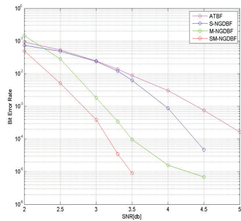
Fig 3. BER performance of bit flipping algorithms: regular LDPC code (PEGReg504 \times 1008 [8])
