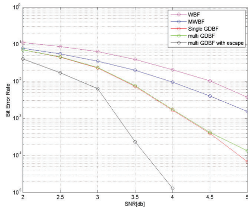
Fig 1. BER performance of bit flipping algorithms: regular LDPC code (PEGReg504 \times 1008 [8])
