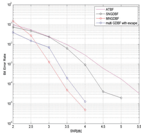
Fig 2. BER performance of bit flipping algorithms: regular LDPC code (PEGReg504 \times 1008 [8])
