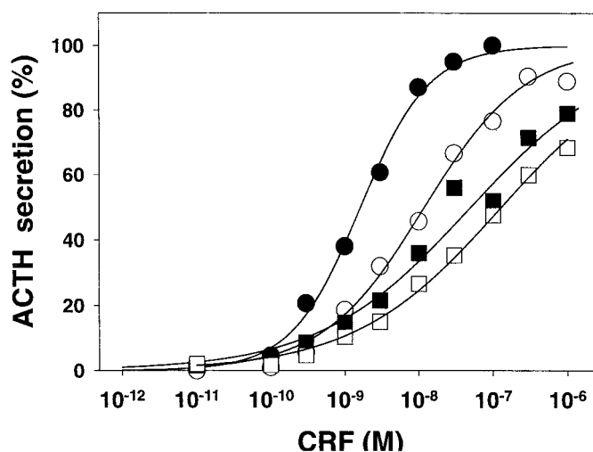
Fig. 3. Antagonism by SSR125543A of CRF-induced ACTH secretion in AtT-20 cells. Concentration-response curves for CRF-stimulated ACTH secretion in AtT-20 cells in the absence (●) or presence of SSR125543A at 3 nM (○), 30 nM (■), and 100 nM (□). The results are expressed as percentage of increase induced by CRF in the presence or absence of SSR125543A. The data are the means of three independent experiments.
