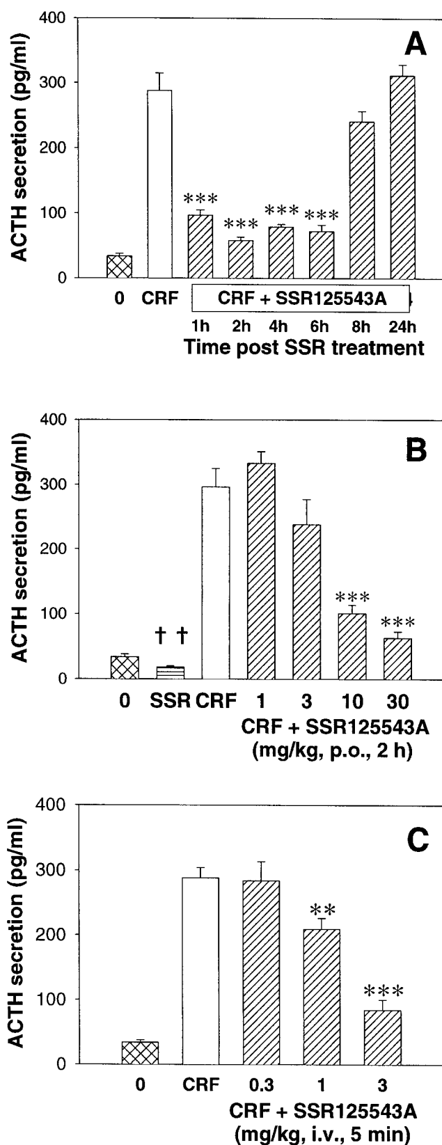
Fig. 5. Effects of SSR125543A on CRF-stimulated ACTH secretion in awake rats. A , time course of the inhibition by SSR125543A of ACTH secretion induced by CRF (4 \mu g/kg i.v.). The compound was administered orally, at the dose of 30 mg/kg, at various time periods (1, 2, 4, 6, 8, and 24 h) before the CRF challenge. B , dose-dependent inhibition induced by oral administration of SSR125543A on ACTH secretion stimulated by CRF injection (4 \mu g/kg i.v.). Increasing doses of SSR125543A (1–30 mg/kg)
