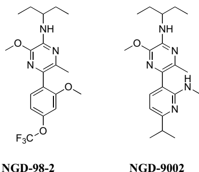
Fig. (2). Structures of pyrazine CRF antagonists.
