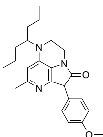
Fig. (11). Structure of Triazaacenaphthylene CRF antagonists.
