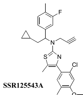
Fig. (5). Structures of thiazole CRF antagonist.
