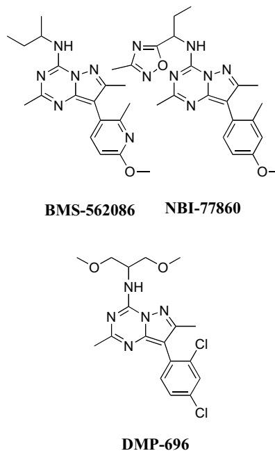
Fig. (7). Structures of Pyrazolo[1,5-a]1,3,5-triazine CRF antagonists.
