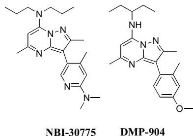
Fig. (8). Structures of Pyrazolo[1,5-a]pyrimidine CRF antagonists.
