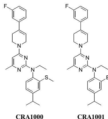
Fig. (4). Structures of pyrimidine CRF antagonists.
