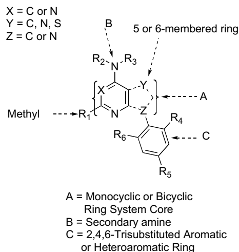
Fig. (1). Pharmacophore structure of CRF1 antagonists.
