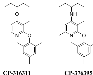
Fig. (3). Structures of pyridine CRF antagonists.
