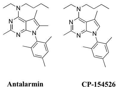
Fig. (6). Structures of Pyrrolo[2,3-d]pyrimidine CRF antagonists.
