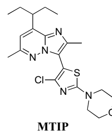
Fig. (10). Structures of Imidazo[1,2-b]pyridazines CRF antagonists.
