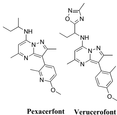
Fig. (9). Structures of Pyrazolo[1,5-a]pyrimidines Verucerofont and Pexacerfont.
