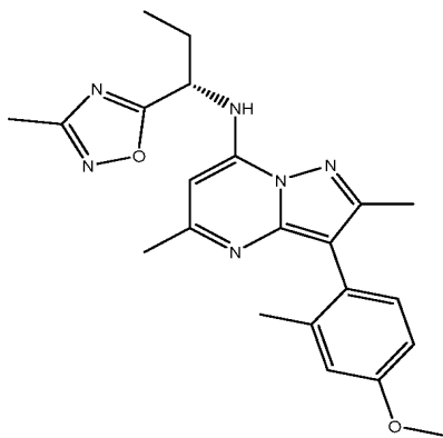
Compound I
