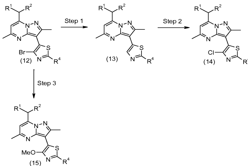
Scheme 3
