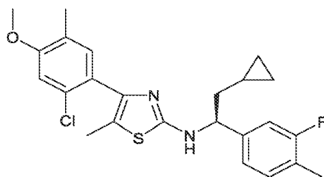
Compound 7-A
