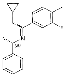
Compound 3-A
