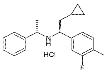
Compound 4-A
