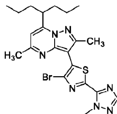
Compound 1.
