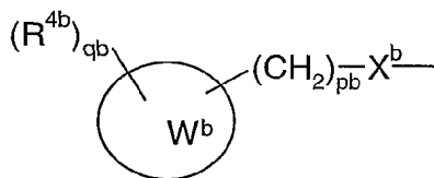
Formula (IIb)
