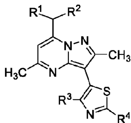
Formula (III)
