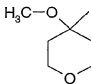
Formula (IIIa)
