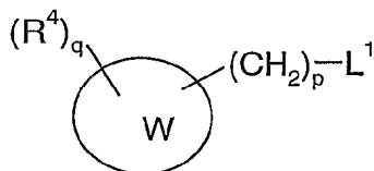
Formula (A)
