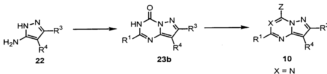
SCHEME 7
