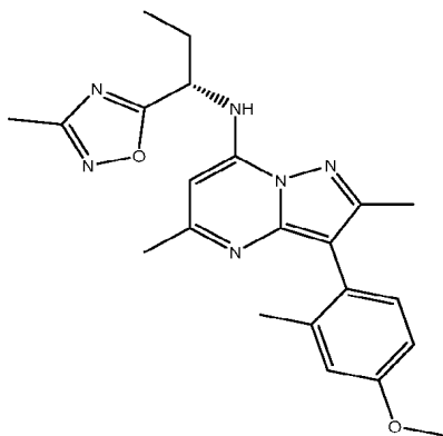
Compound I
