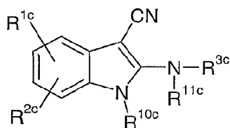
Formula (Ic)
