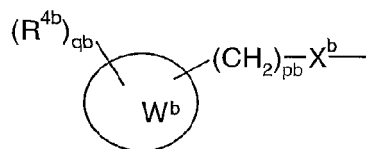
Formula (IIb)
