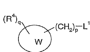
Formula (A)
