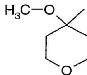
Formula (III)
