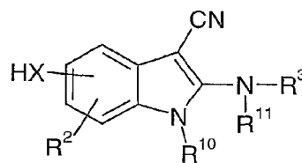
Formula (B)
