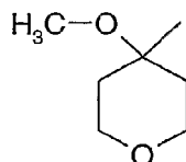
Formula (IIIa)
