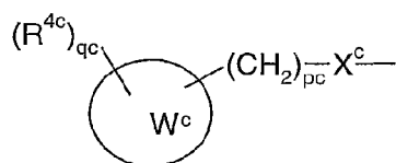
Formula (IIc)
