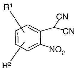
Formula (C)
