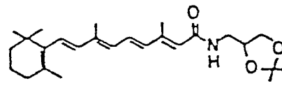
N-Methyl-dimethyldioxolan-retinamide
