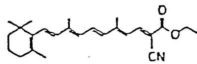
Retinylidene ethylcyano-
