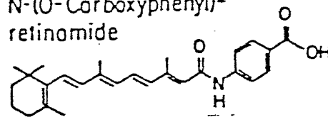
N-(p-Carboxyphenyl)-retinamide
