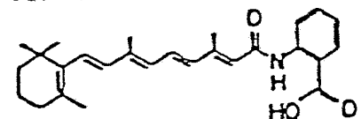
N-(O-Carboxyphenyl)-retinamide
