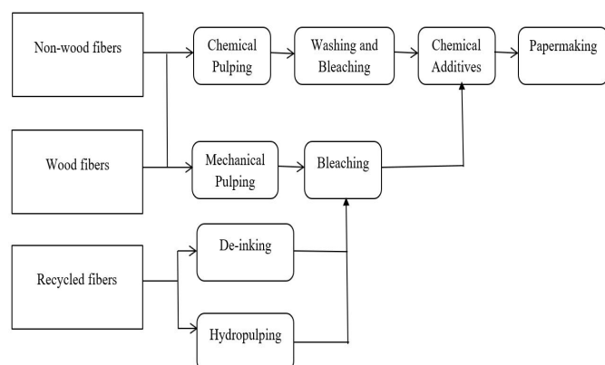
Figure 1: Papermaking process of different raw material.
