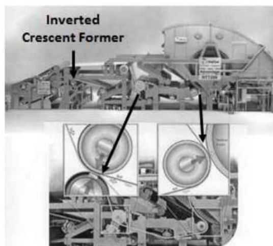
Fig. 8. New tissue technology (NTT) machine (Valmet 2014)
