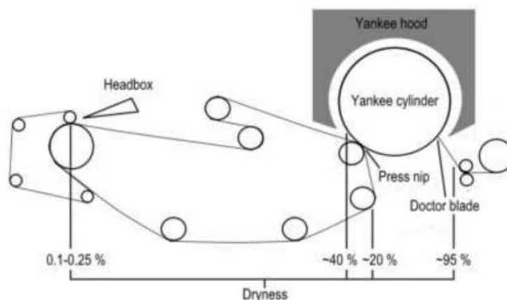
Fig. 1. Sketch of light dry crepe (LDC) tissue machine composed by a crescent former, pressing section, Yankee cylinder and creping blade (Tysén 2014)
