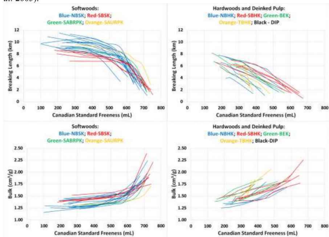
Fig. 11. Breaking length and bulk, as a function of freeness. NBSK: northern bleached softwood kraft; SBSK: southern bleached softwood kraft; SABRPK: South American bleached radiata pine kraft; SAURPK: South American unbleached radiata pine kraft; NBHK: northern bleached hardwood kraft; SBHK: southern bleached hardwood kraft; BEK: bleached eucalyptus kraft; TBHK = tropical bleached hardwood kraft; DIP: deinked pulp (Adapted from Nanko et al. 2005)
