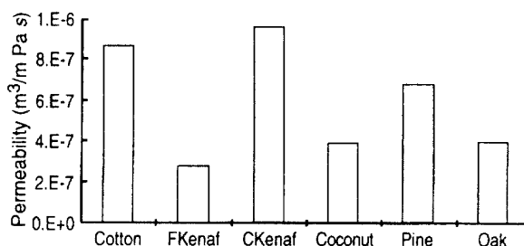
Fig. 9. Permeability values of some common nonwood fibers.
