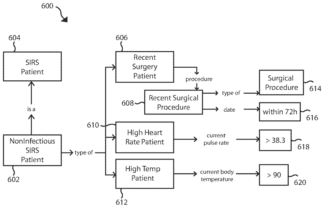
Automatically Generated First Order Logic Rules Snippets
