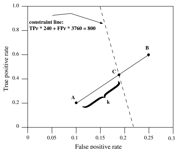
Fig. 10. Interpolating classifiers.
